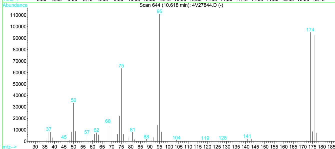
Spectrum Information: Scan 644
