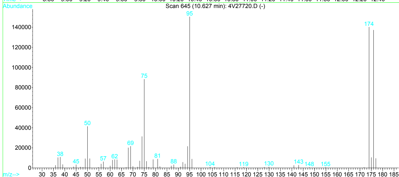
Spectrum Information: Scan 645
