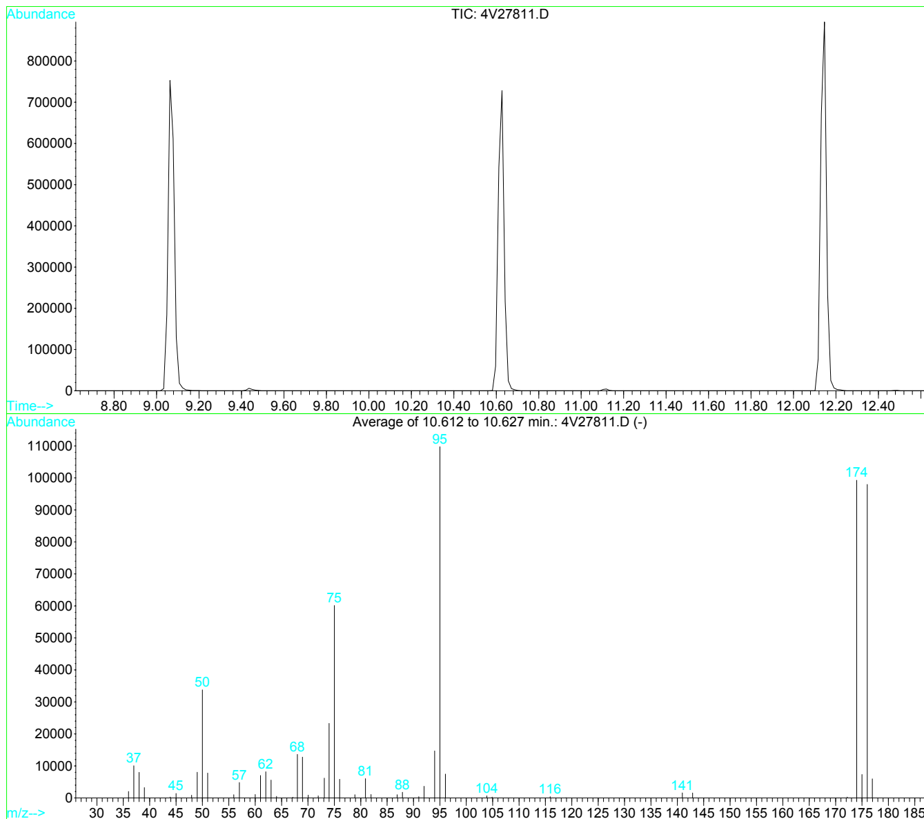
Spectrum Information: Average of 10.612 to 10.627 min.
