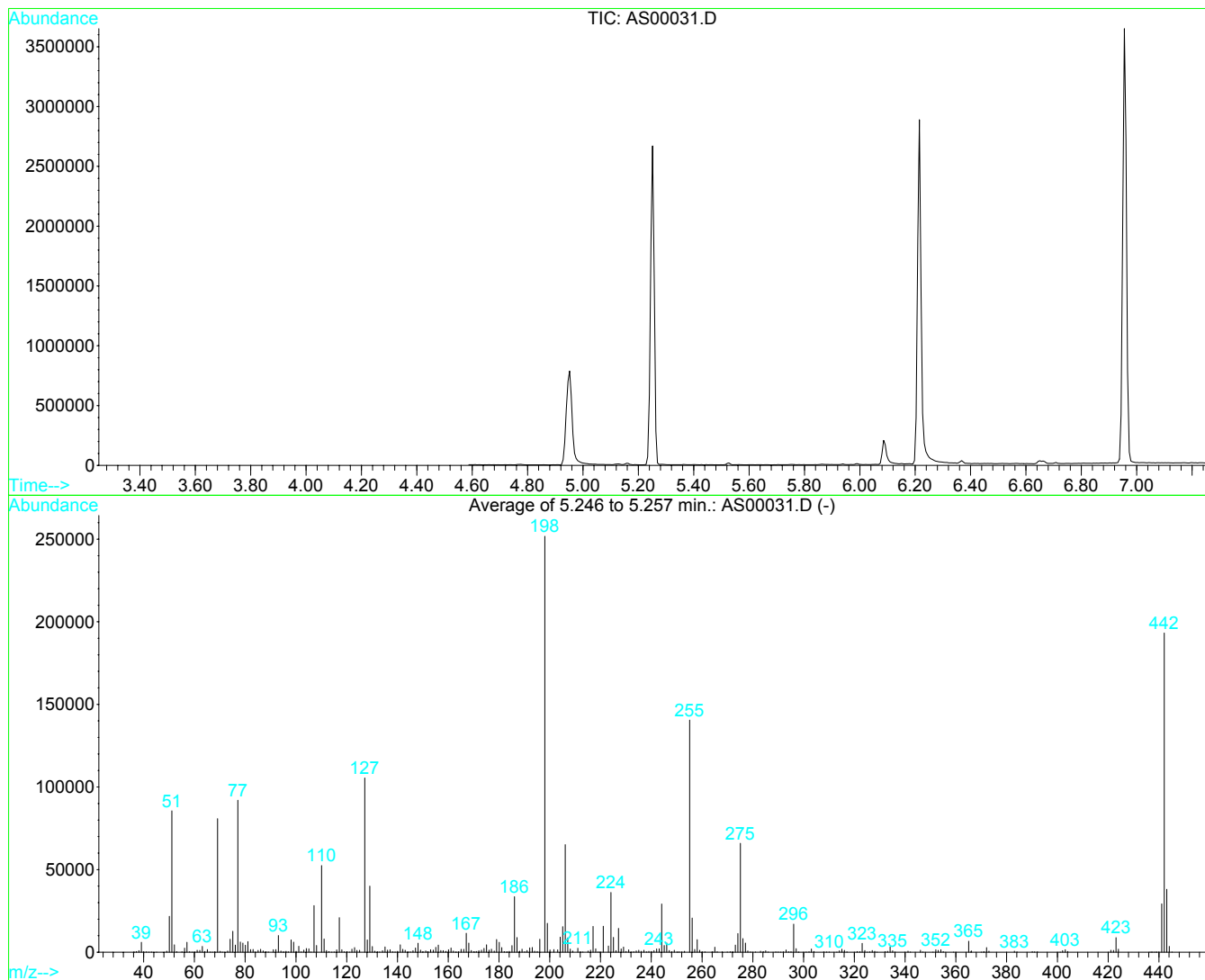
Spectrum Information: Average of 5.246 to 5.257 min.
